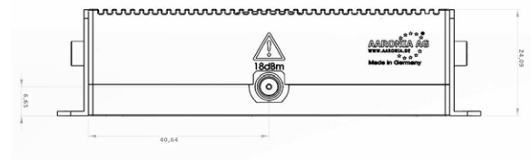
Side view BPSG OEM versions
