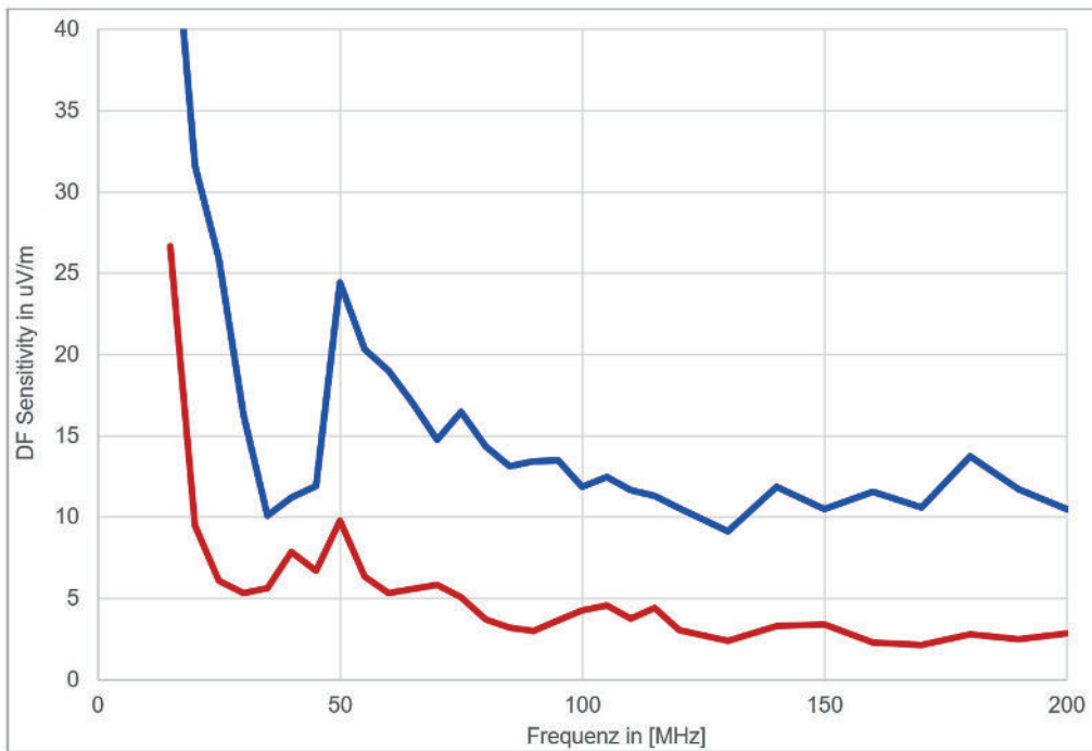
Fig. 12. DF sensitivity for 3° RMS bearing fluctuation according to ITU-R SM.2096-0 Blue curve: CBW 1 kHz, Avg. Time 1 s; Red curve: CBW 600 Hz, Avg. Time 5 s
