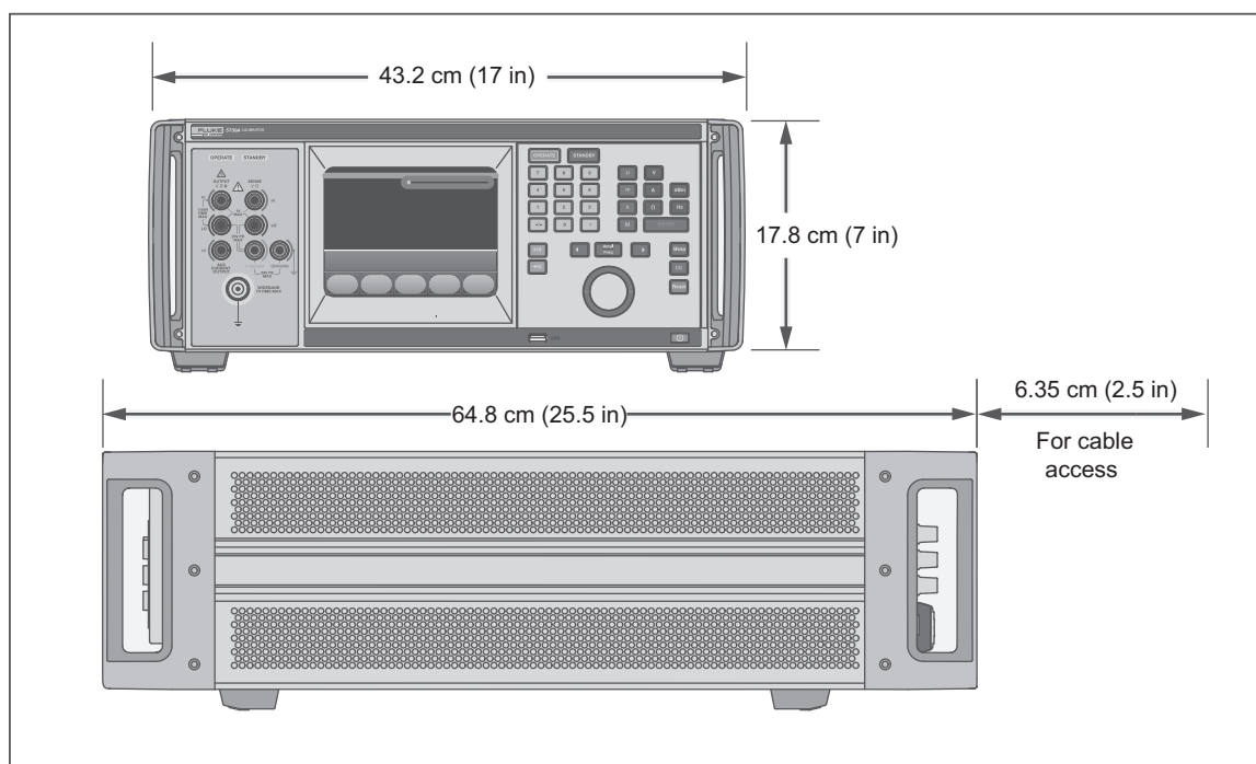
Figure 1-1. Product Dimensions
