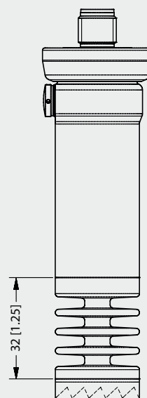
P41 | High-temperature version with cooling section
