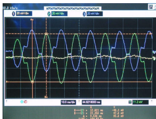
The oscilloscope display shows the welding current when using the analog signal output of ELT-400
