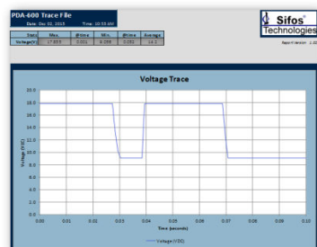
Figure 4: 2-Event Classification
