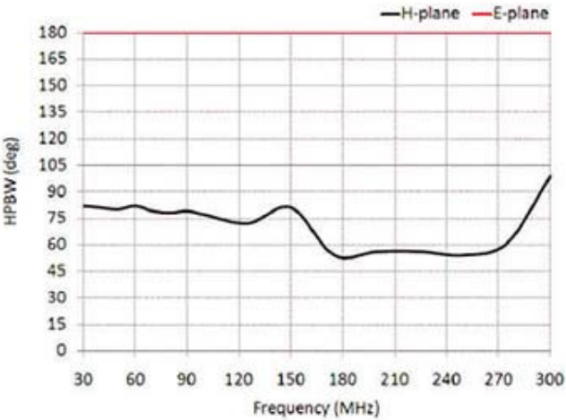
3110C Biconical Antenna Beamwidth Typical Measured Data
