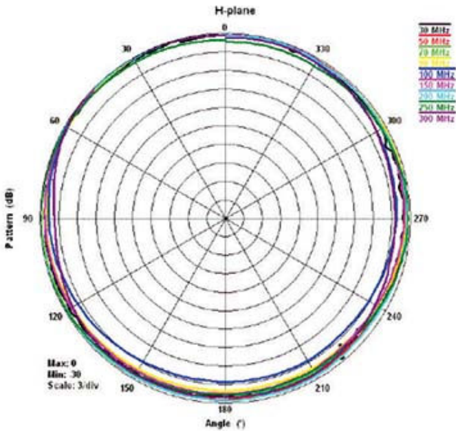
3110C H-Plane 30 MHz to 300 MHz
