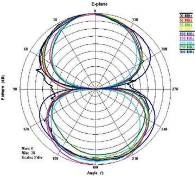
3110C E-Plane 30 MHz to 300 MHz
