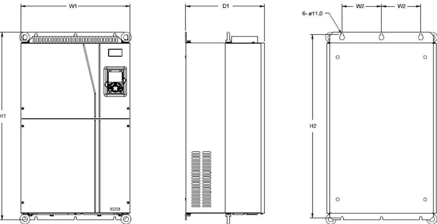
Wall installation diagram of VFDs of 460V 132-200kW/175-270HP
