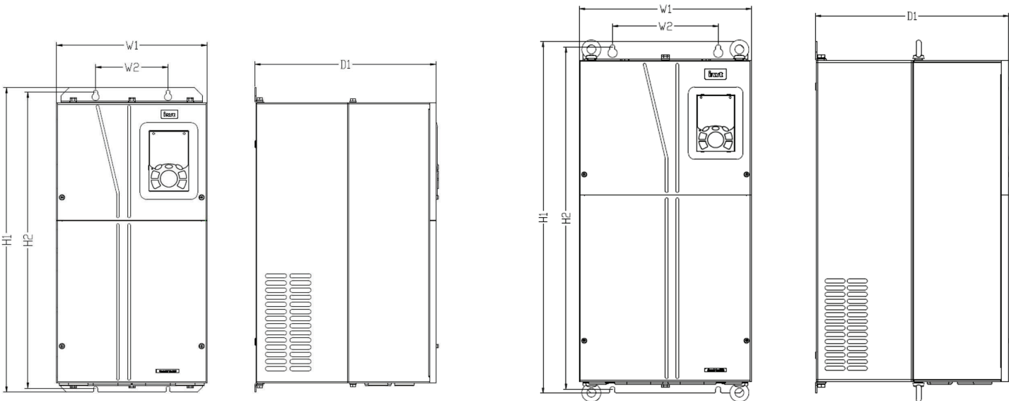
Wall installation diagram of VFDs of 220V 18.5-55kW/25-75HP and 460V 37-55kW/50-75HP Wall installation diagram of VFDs of 460V 75-110kW/100-150HP
