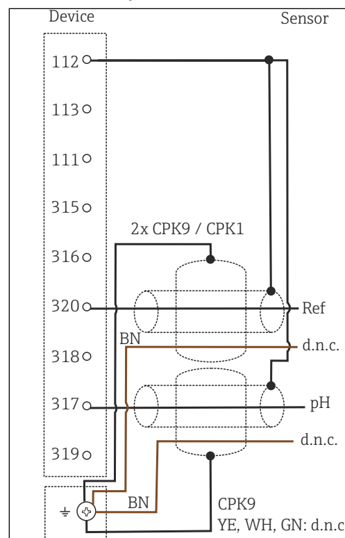
39 Wiring diagram
