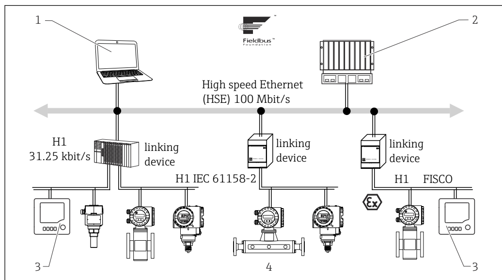
66 System architecture with associated components
