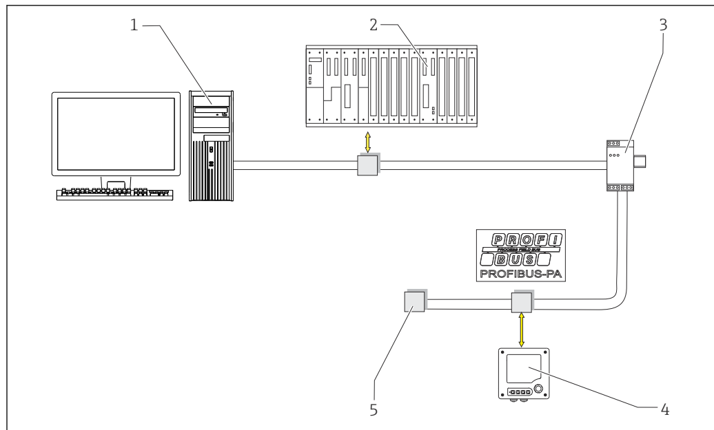
65 PROFIBUS system integration
