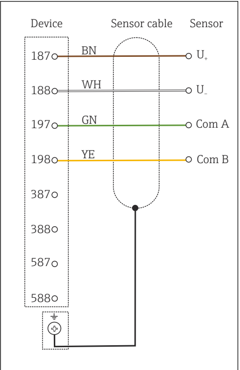
23 Wiring diagram
