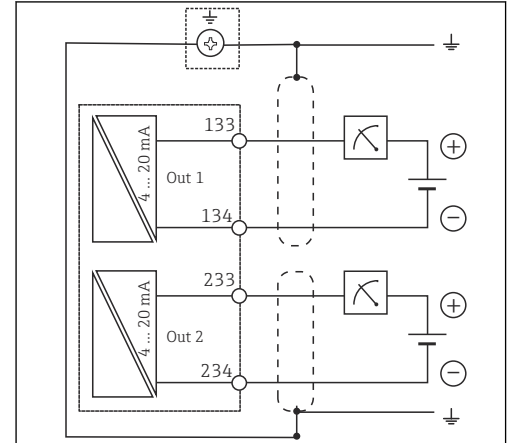
13 Wiring diagram
