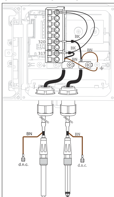
38 In-device view (sensor module)
