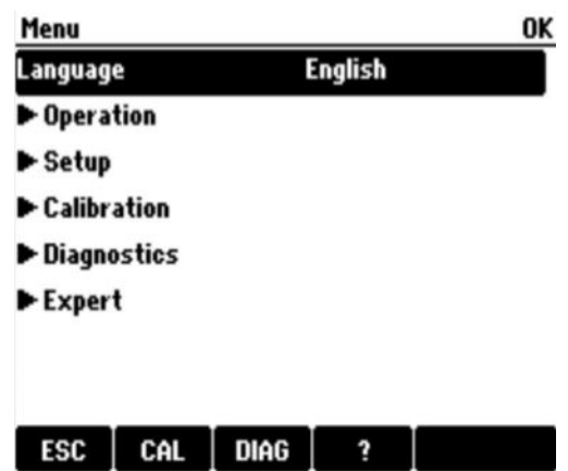
38 Plain-text menu
