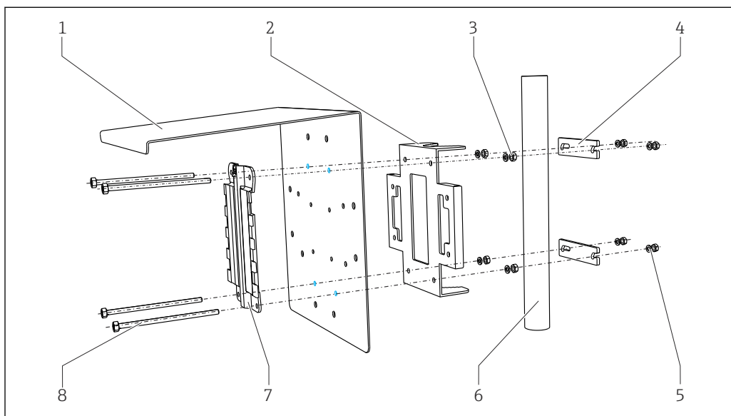
32 Post mounting
