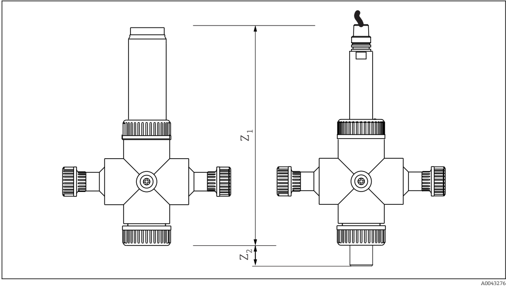
7 Adapter in standard version (left) and version for CAS80E (right)
