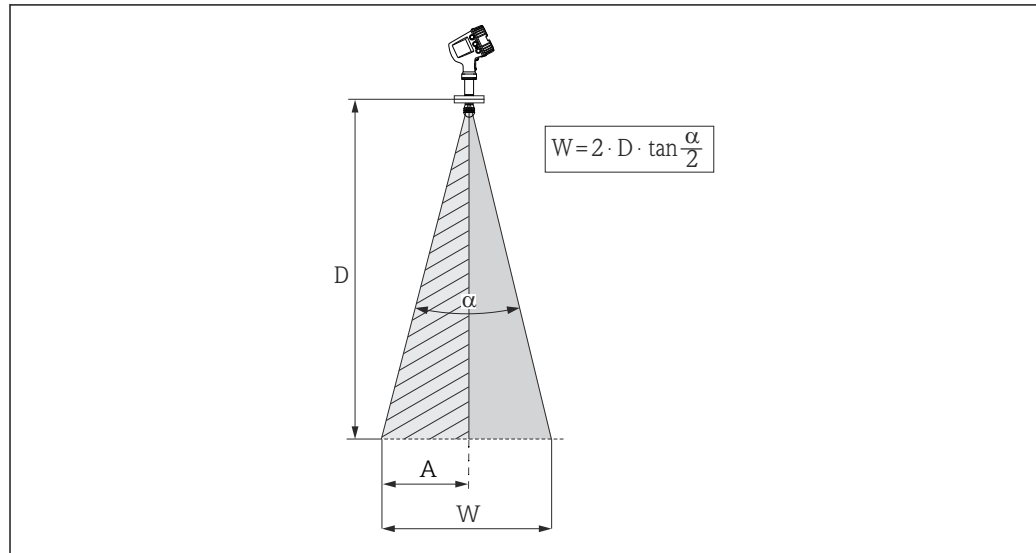
12 Relationship between beam angle \alpha , distance D and beam diameter W . Distance A is the minimum distance to the tank wall (or other installations). Distance A equals the half of beam diameter W
