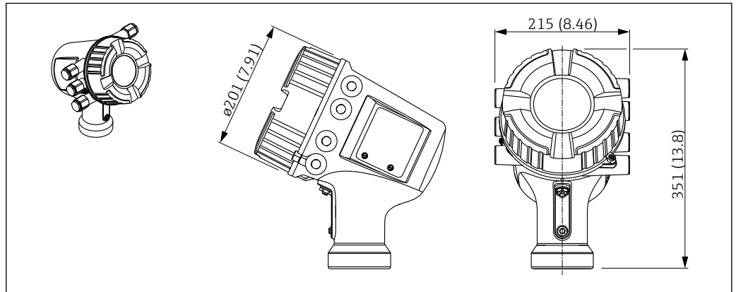
14 Dimensions of the electronics housing; unit of measurement: mm (in); adapters for cable entries are not taken into account in this drawing.
