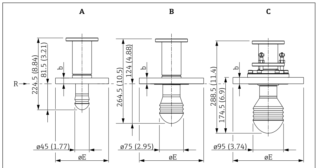
15 Antenna size; unit of measurement: mm (in)
