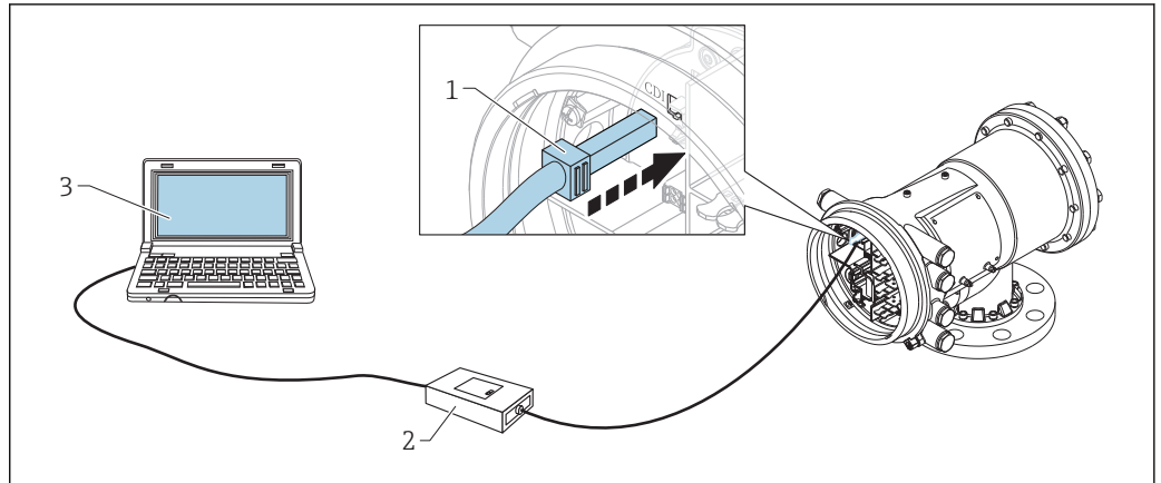
22 Operation via service interface
