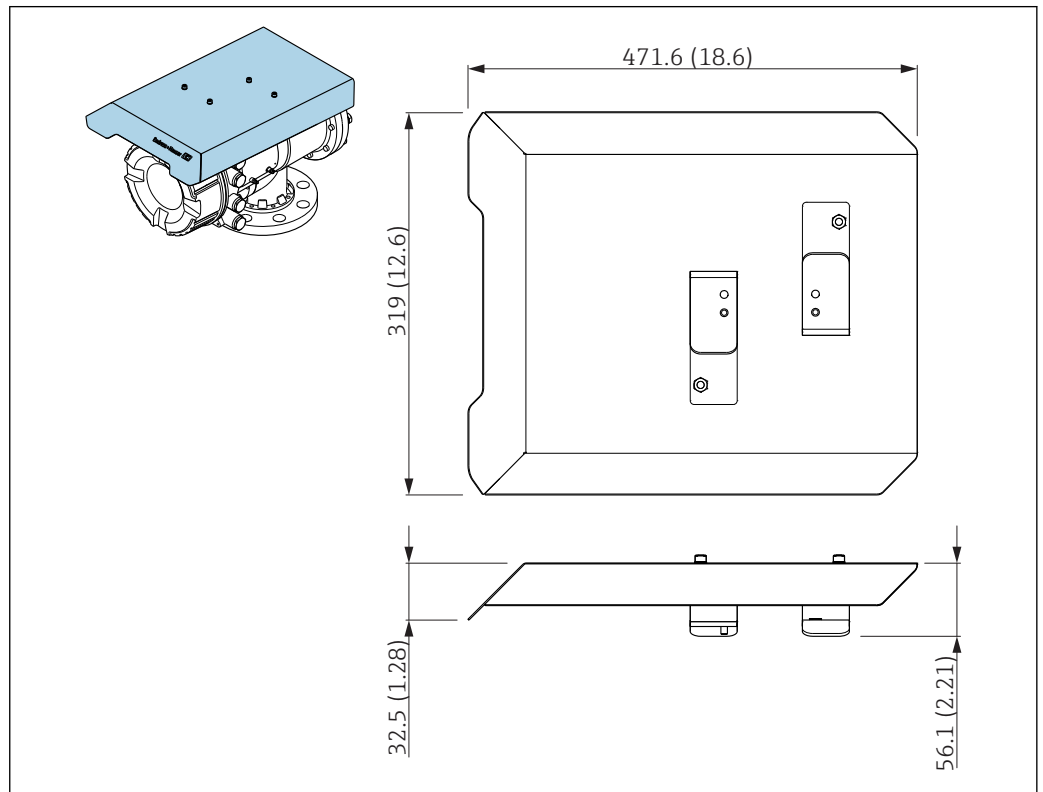
24 Weather protection cover; dimensions: mm (in)
