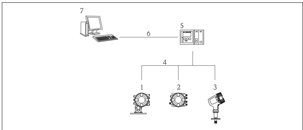
21 Remote operation of Tank Gauging devices
