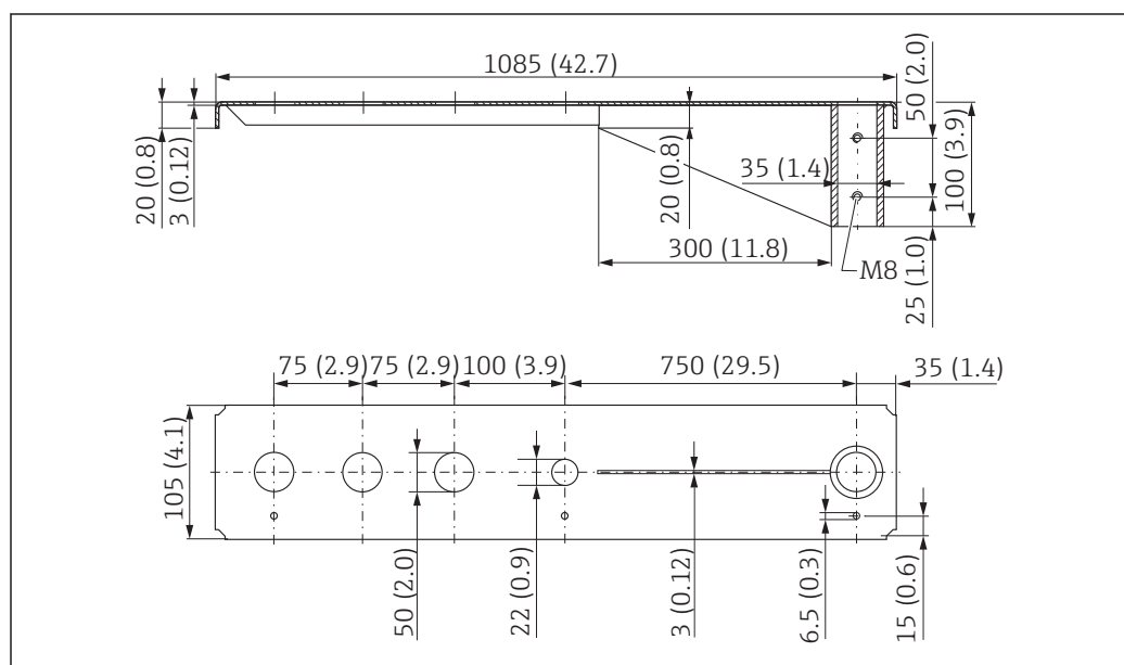
35 Dimensions of cantilever (long) with pivot for G 1-½" sensor process connection on front. Unit of measurement mm (in)
