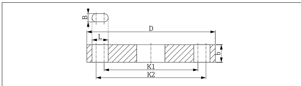
28 Dimensions of the UNI flange FAX50
