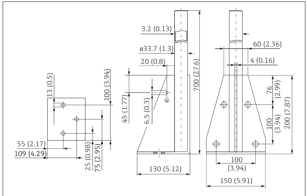
36 Dimensions of mounting frame (short). Unit of measurement mm (in)
