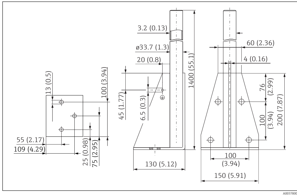
37 Dimensions of mounting frame (long). Unit of measurement mm (in)
