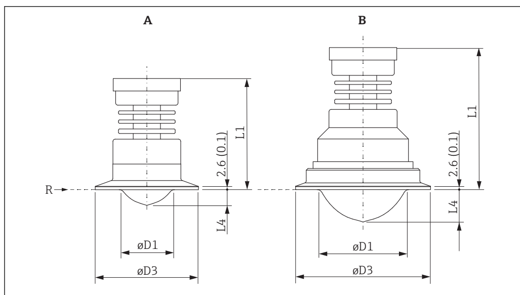
36 Dimensions of device with Tri-Clamp connection. Unit of measurement mm (in)
