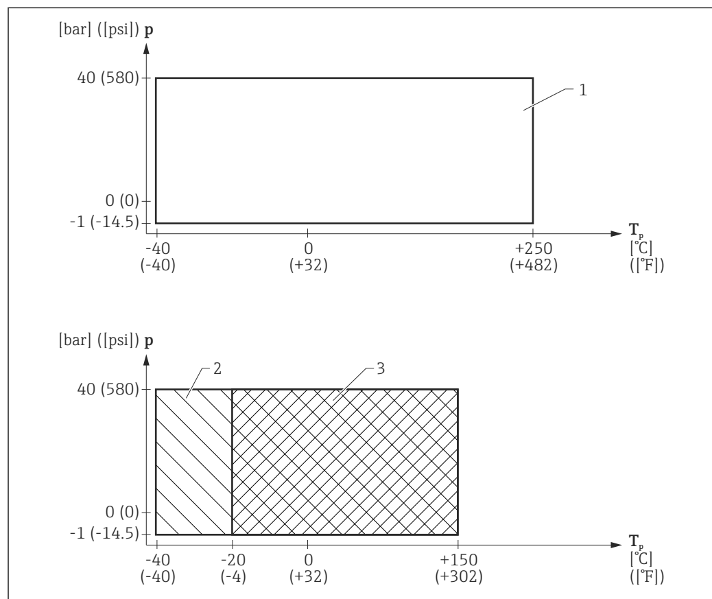
25 FMR51: Permitted range for process temperature and process pressure
