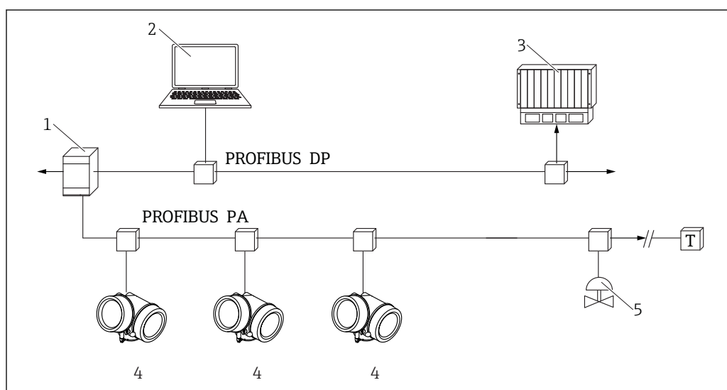
42 Options for remote operation via PROFIBUS PA protocol
