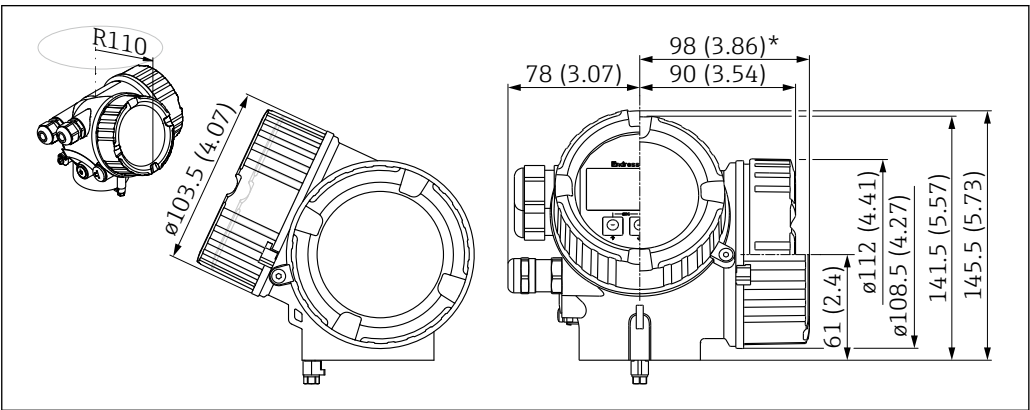
30 Housing GT20 (aluminum coated). Unit of measurement mm (in)
