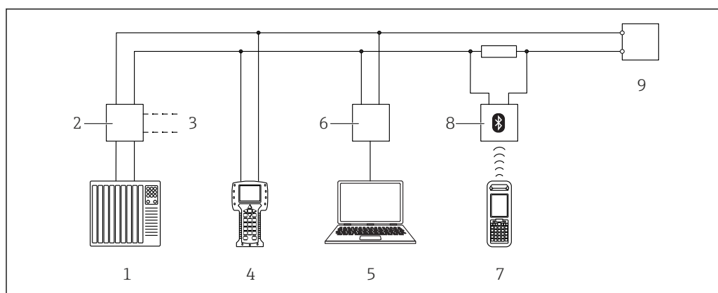
41 Options for remote operation via HART protocol
