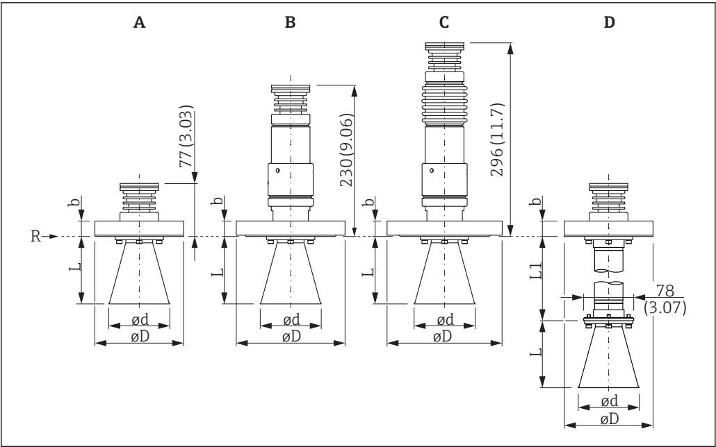
31 Dimensions of FMR54 with horn antenna. Unit of measurement mm (in)
