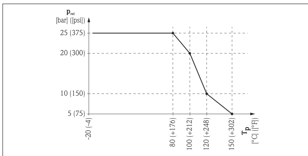
25 FMR54 with planar antenna: Permitted range for process temperature and process pressure
