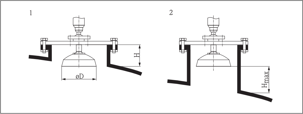
23 Nozzle mounting of Micropilot FMR57 with parabolic antenna
