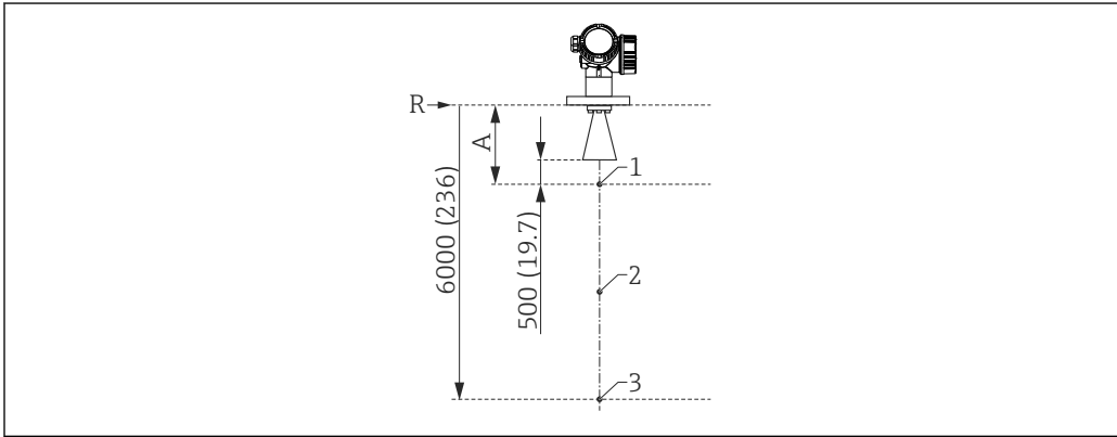
48 Points of the 3-point linearity protocol; engineering unit: mm (in)
