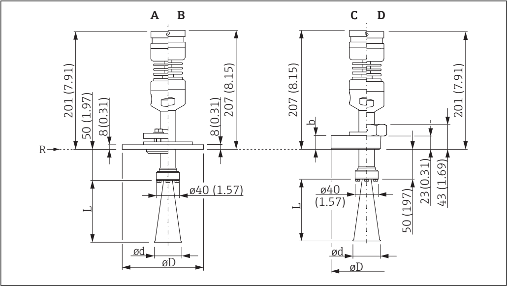
37 Dimensions of FMR57 with horn antenna - high-temperature version; engineering unit: mm(in) A Process connection: alignment unit with UNI flange B Process connection: UNI flange C Process connection: flange D Process connection: thread MNPT1-1/2 or R1-1/2 R Reference point of measurement ØD As per flange standard ASME B16.5 / EN1092-1 / JIS B2220 b As per flange standard ASME B16.5 / EN1092-1 / JIS B2220
