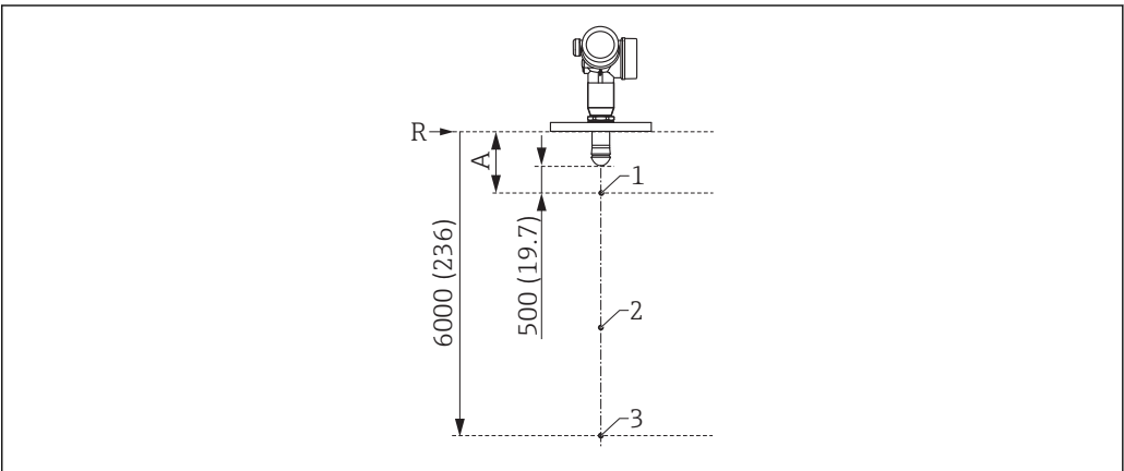
28 Points of the 3-point linearity protocol. Unit of measurement mm (in)
