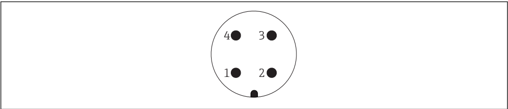
22 Pin assignment of M12 plug
