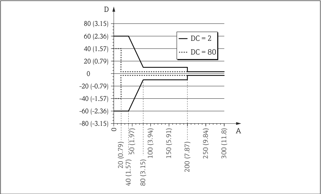
24 Measured error at the probe end for rod and coax probes A Distance from the probe end [mm(in)] D Measured error: Sum of non-linearity, non-repeatability and hysteresis
