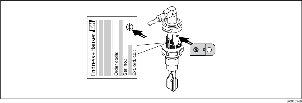
23 Position for test magnet on housing
