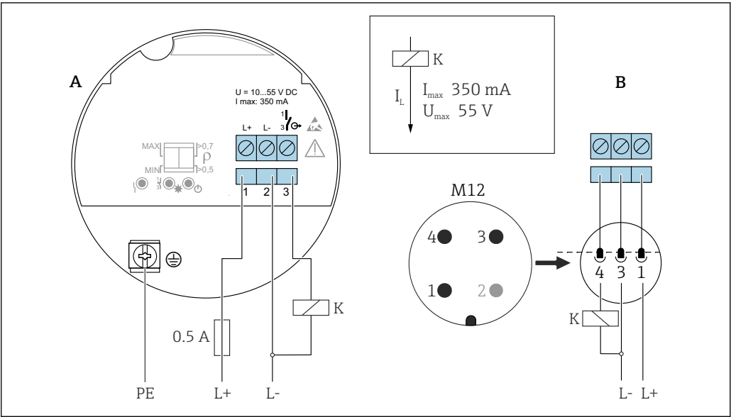
2 FEL42 terminal assignment A Terminal assignment at electronic insert B Terminal assignment on M12 plug
