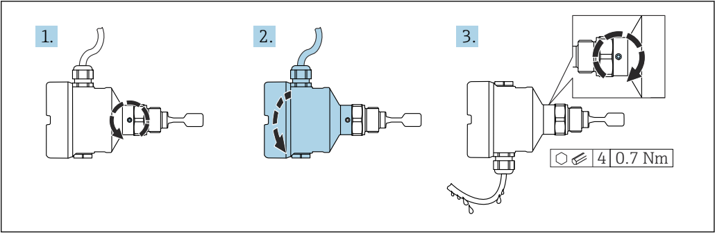
17 Housing with external locking screw
