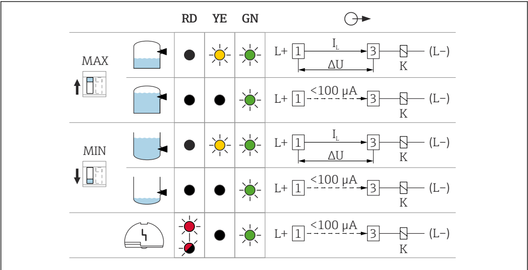
3 FEL42 switching behavior, signaling LED MAXDIP switch for setting the MAX safety MIN DIP switch for setting the MIN safety RD LED red for warning or alarm YE LED yellow, switch status GN LED green, operational status, device on I_L Load current switched through
