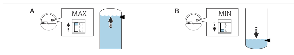
41 Switch position on the electronic insert for MAX/MIN safety mode
