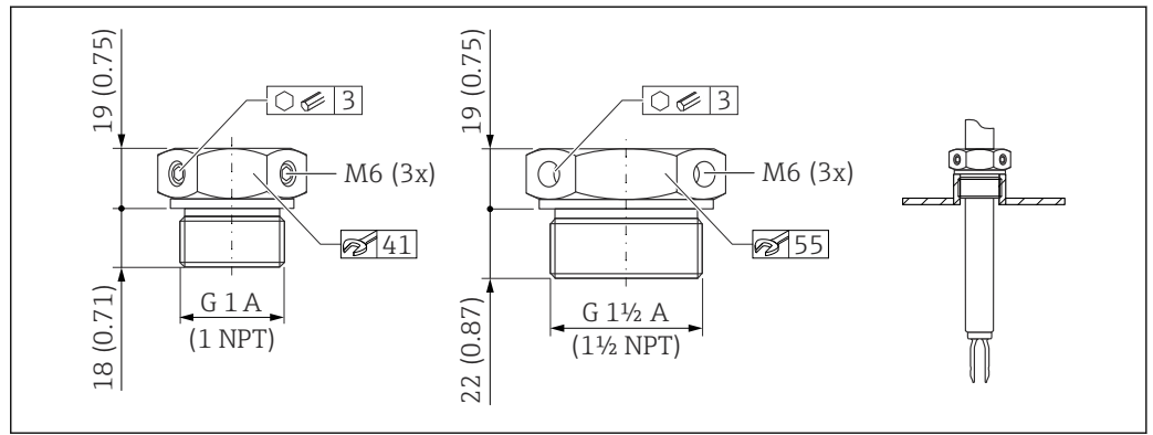
41 Sliding sleeves for unpressurized operation p_e = 0 bar (0 psi). Unit of measurement mm (in)
