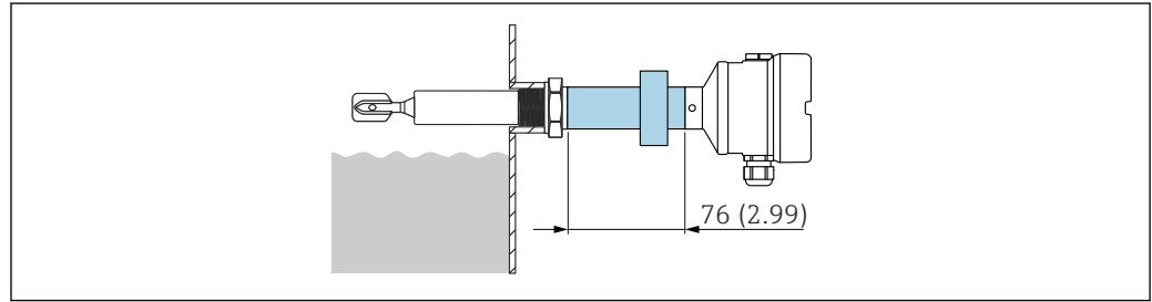
20 Ex d glass feedthrough for pipe extensions . Unit of measurement mm (in)
