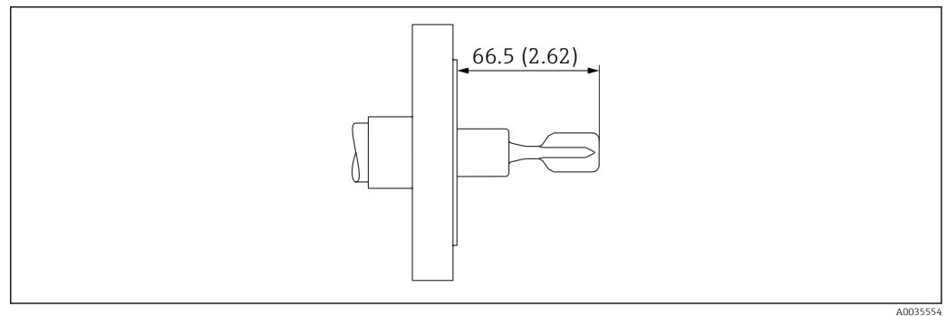
34 Example with flange. Unit of measurement mm (in)
