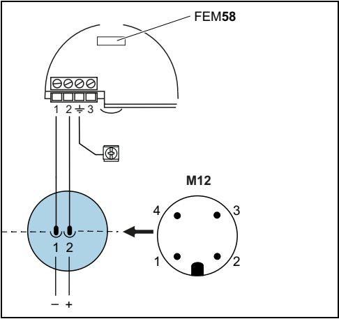
With M12 plug wired at the factory (Ordering feature 80, option 1)
