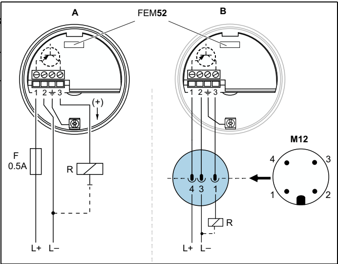
DC: U = 10 \text{ V} \dots 55 \text{ V} A: With cable entry wired by customer (Ordering feature 80, options 2, 3, 4, 7) B: With M12 plug wired at the factory (Ordering feature 80, option 1)
