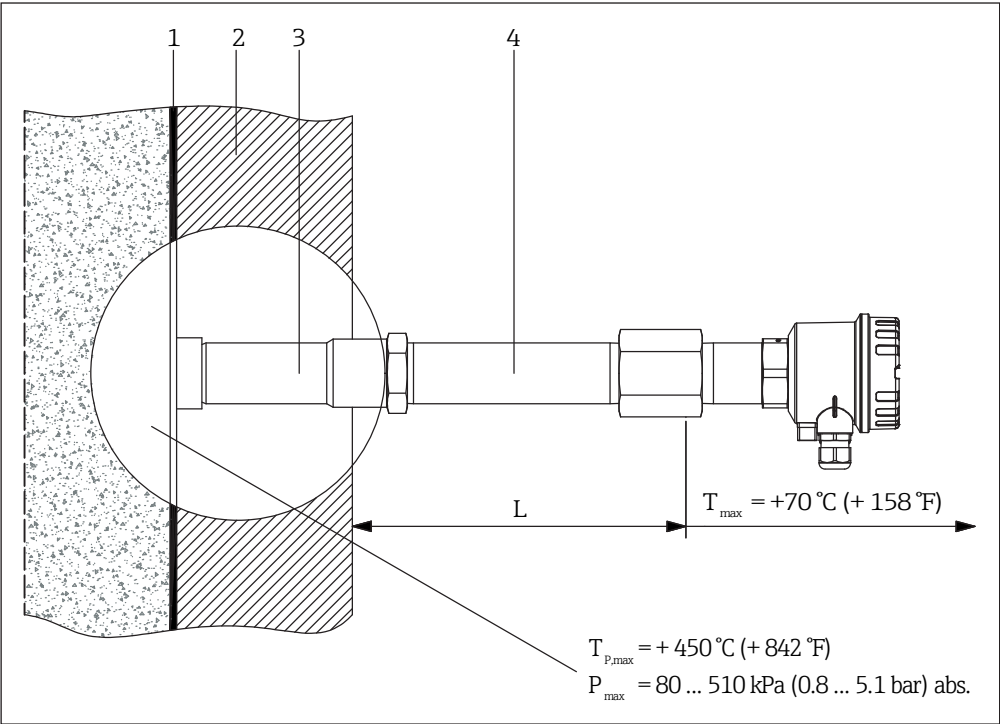
22 Mounting with high temperature adapter and length extensions
