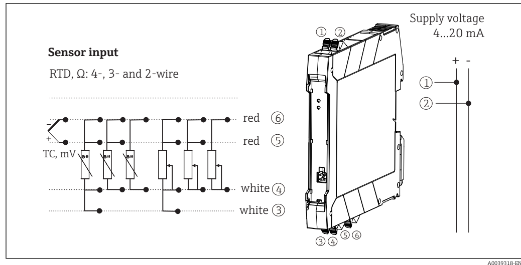
4 Assignment of terminal connections for DIN rail transmitter
