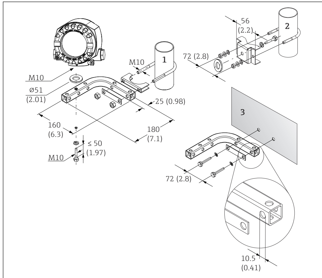
7 Mounting the field mount housing using special mounting bracket. Dimensions in mm (in)
