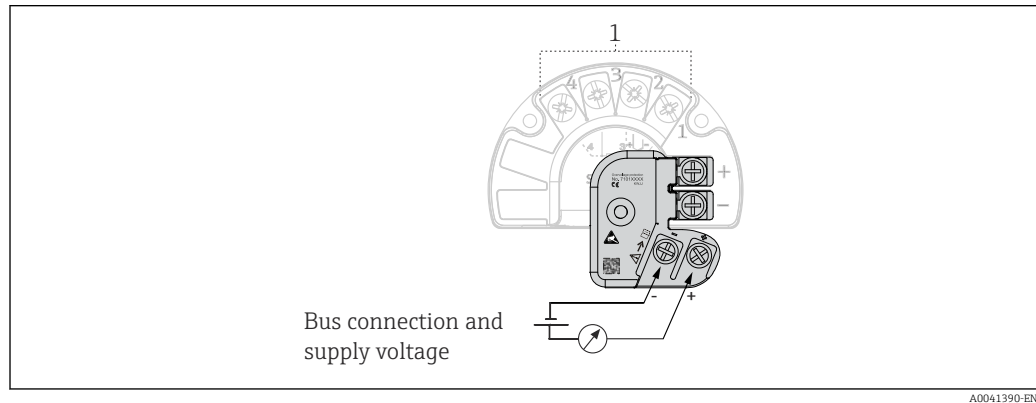
4 Electrical connection of surge arrester
