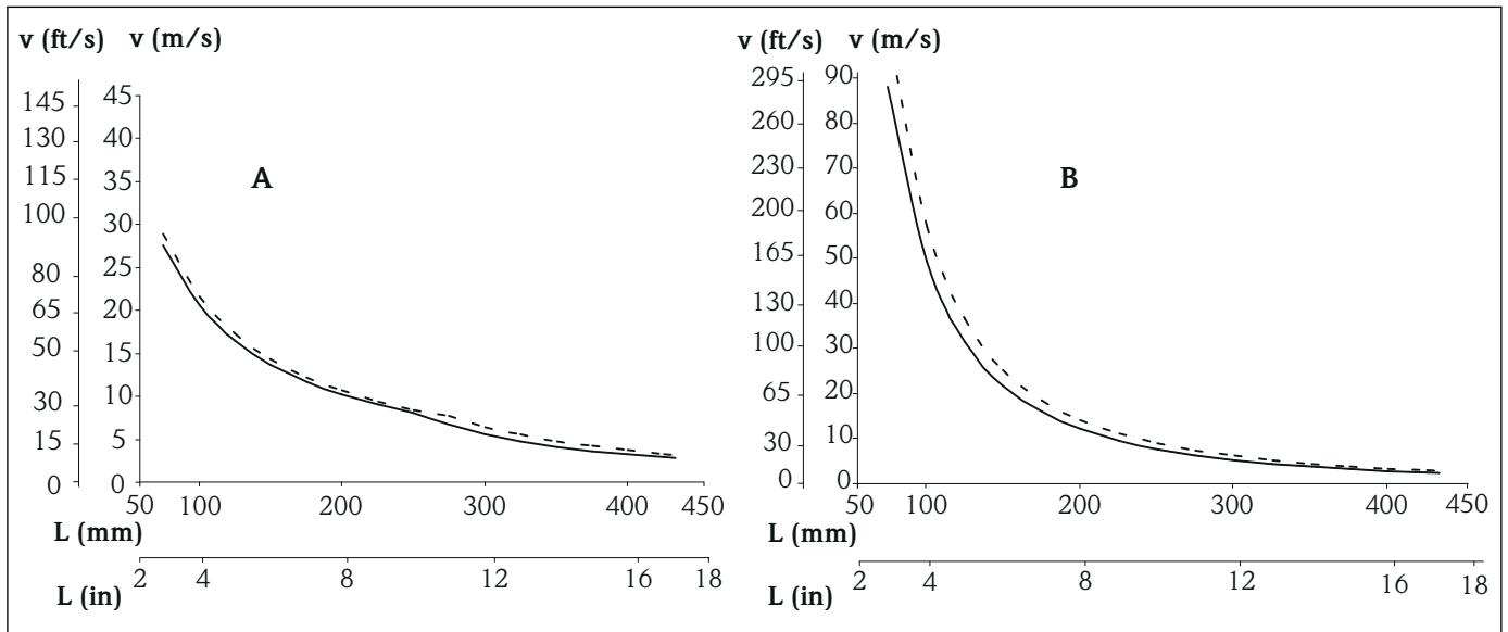
16 Maximum flow velocity with thermowell diameter 14 mm (0.55 in) (—) or 15 mm (0.6 in) (-----)
