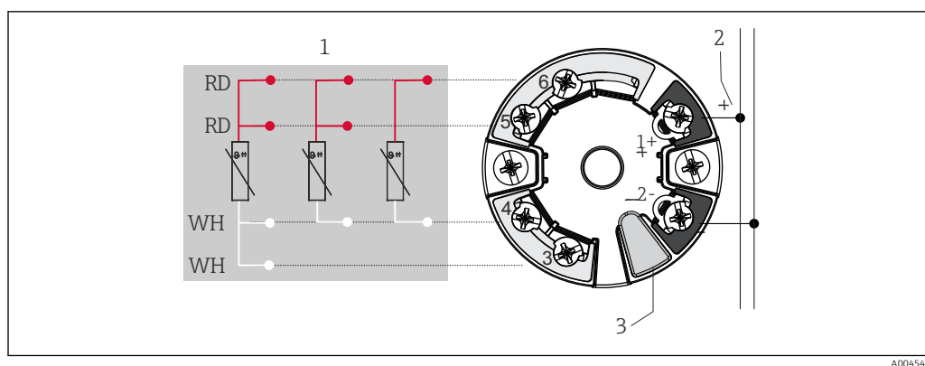
5 Head mounted transmitter TMT7x (single input)
