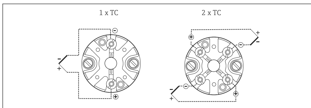
9 Terminal block mounted
