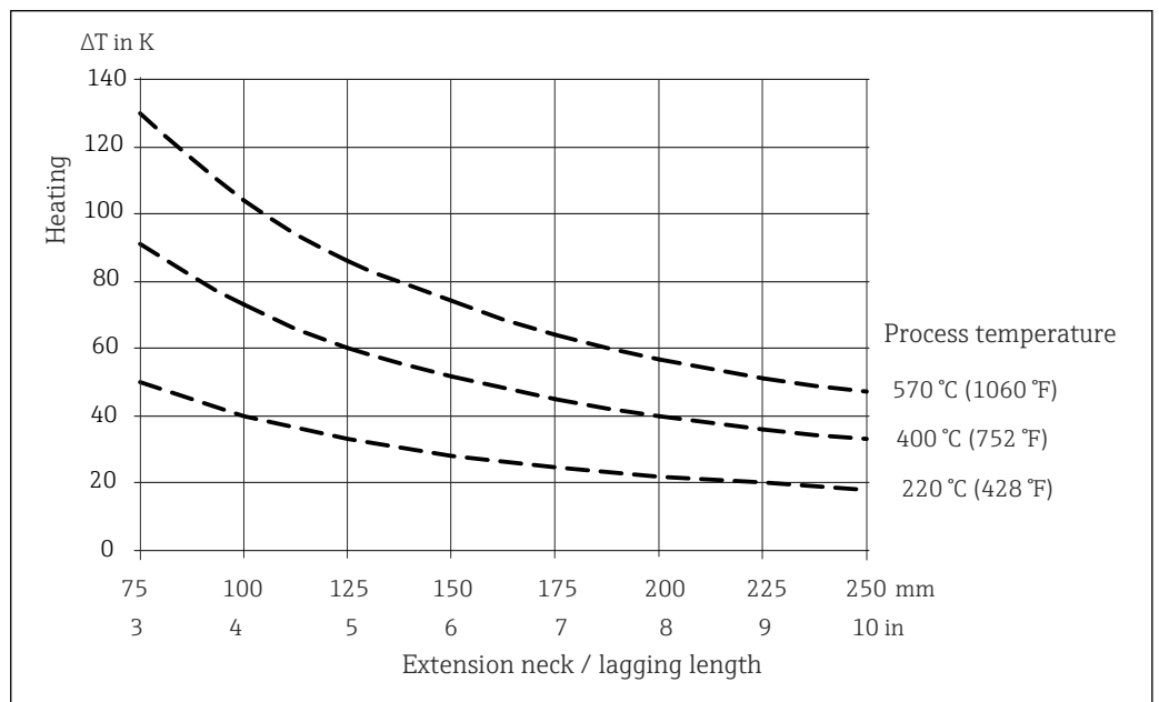
25 Heating of the terminal head as a function of the process temperature. Temperature in terminal head = ambient temperature 20 °C (68 °F) + \Delta T
