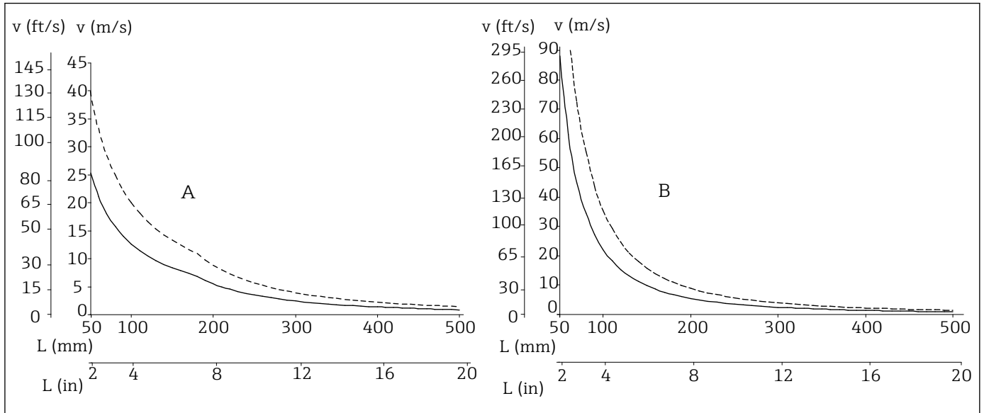
15 Maximum flow velocity with thermowell diameter 9 mm (0.35 in) (—) or 12 mm (0.47 in) (-----)
