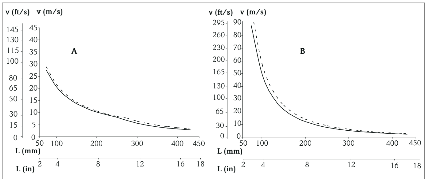
5 Maximum flow velocity with thermowell diameter 14 mm (0.55 in) (—) or 15 mm (0.6 in) (----) A Medium: water at T = 50\text{ }^{\circ}\text{C} (122 ^{\circ}\text{F} ) B Medium: superheated steam at T = 400\text{ }^{\circ}\text{C} (752 ^{\circ}\text{F} ) L Immersion length v Flow velocity
