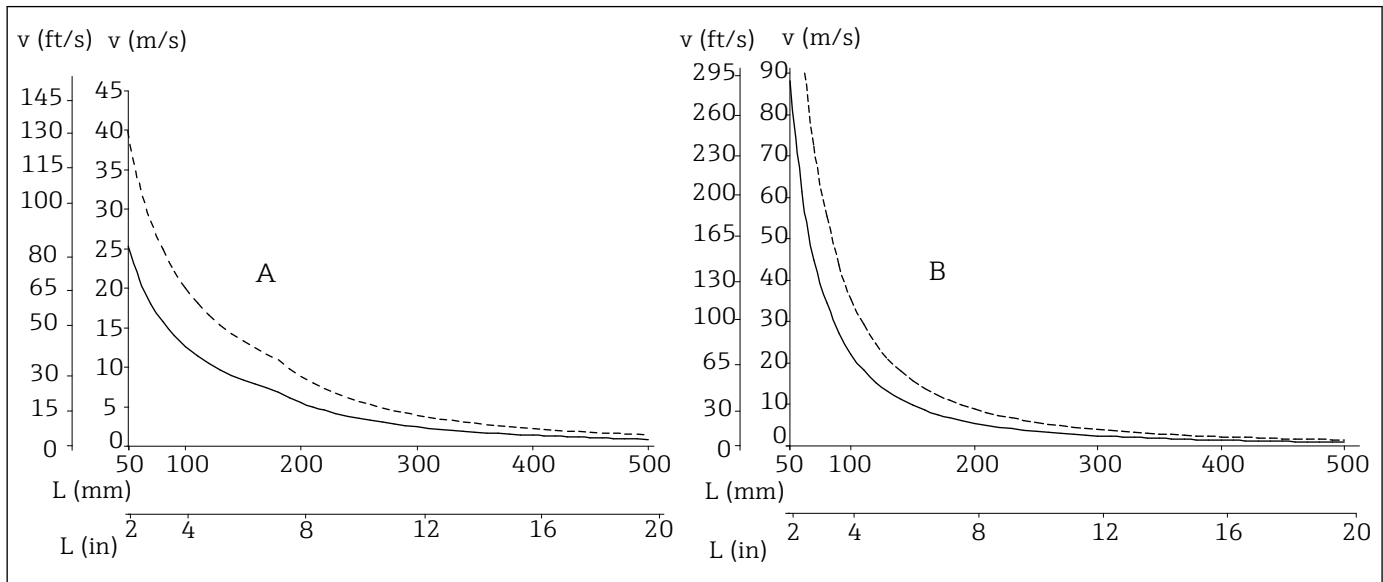
4 Maximum flow velocity with thermowell diameter 9 mm (0.35 in) (—) or 12 mm (0.47 in) (----) A Medium: water at T = 50\text{ }^{\circ}\text{C} (122 ^{\circ}\text{F} ) B Medium: superheated steam at T = 400\text{ }^{\circ}\text{C} (752 ^{\circ}\text{F} ) L Immersion length v Flow velocity
