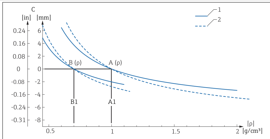
7 Switch point deviation over density
