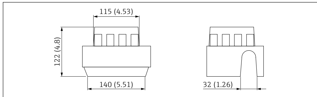
38 Weather protection cover for single compartment housing, aluminum. Unit of measurement mm (in)
