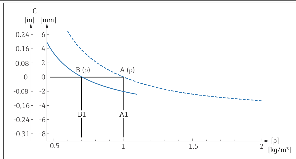
19 Reference switch points via density, plastic coating (ECTFE, PFA)
