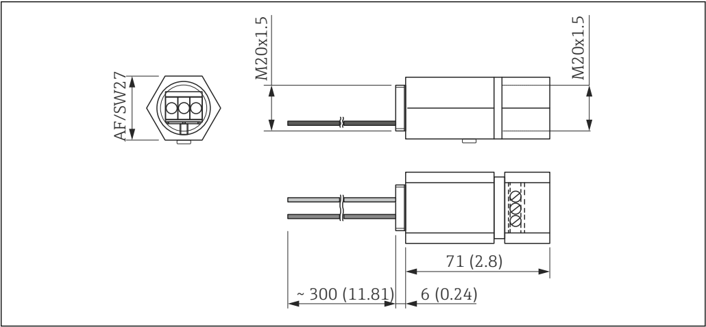
13 Dimensions for HAW569-xA2B in mm (in), surge arrester for protecting signal cables, optionally for protecting intrinsically safe measuring circuits.
