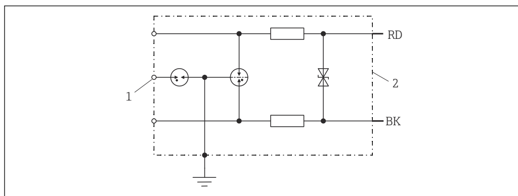
6 Internal circuitry HAW569-AA2B
