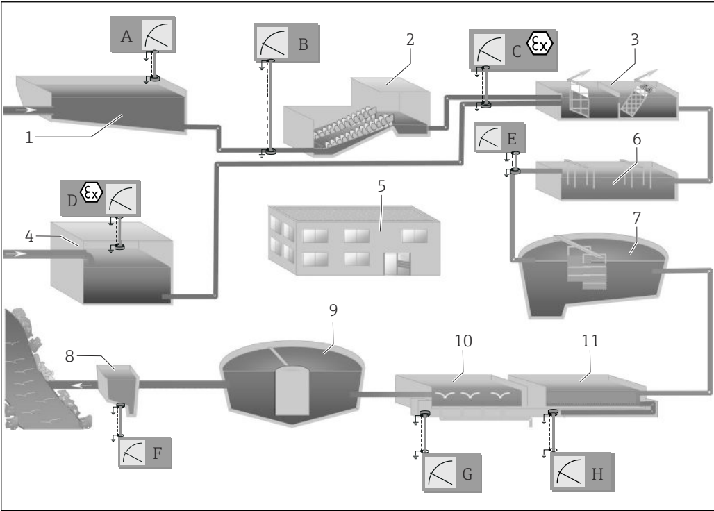
1 Application example: wastewater treatment plant (schematic diagram)
