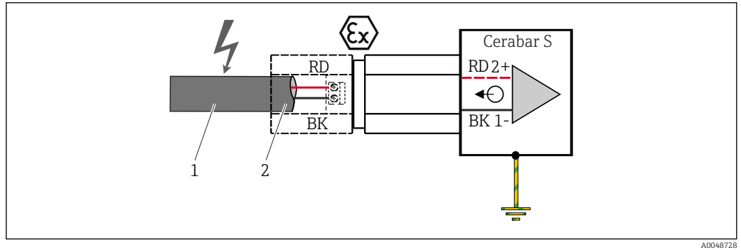
3 Pressure measurement with Cerabar S pressure transmitter
