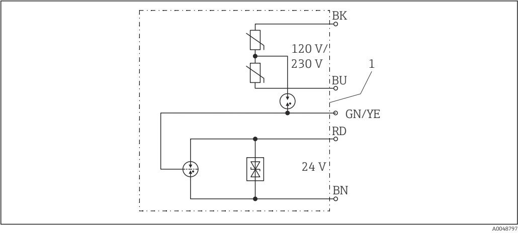
8 Internal circuitry HAW569-CB2C
