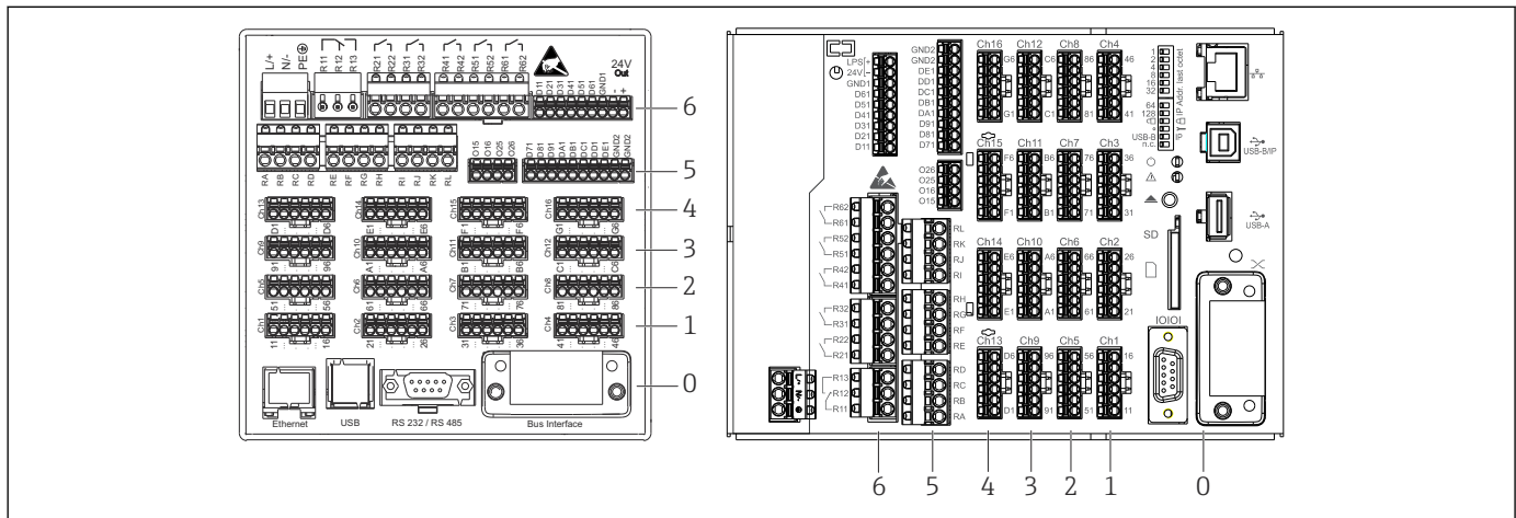
1 Connections: back of device, panel version (left), DIN rail version (right)
