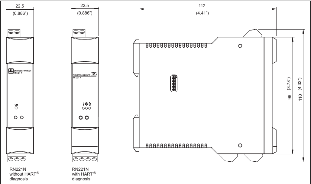
Dimensions of RN221N (data in mm, data in inches in brackets)
