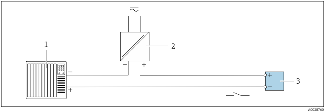
5 Connection example for switch output (passive) 1 Automation system with switch input (e.g. PLC) 2 Power supply 3 Transmitter: Observe input values
