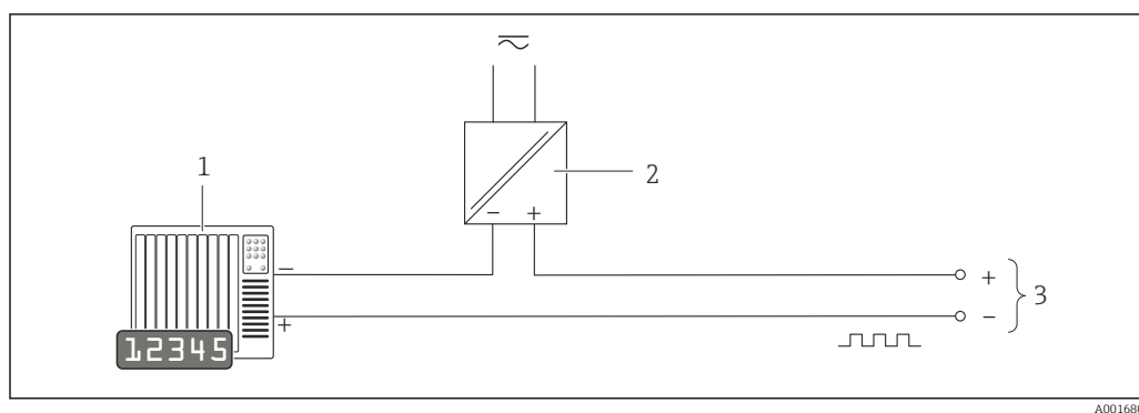
10 Connection example for pulse/frequency output (passive)
