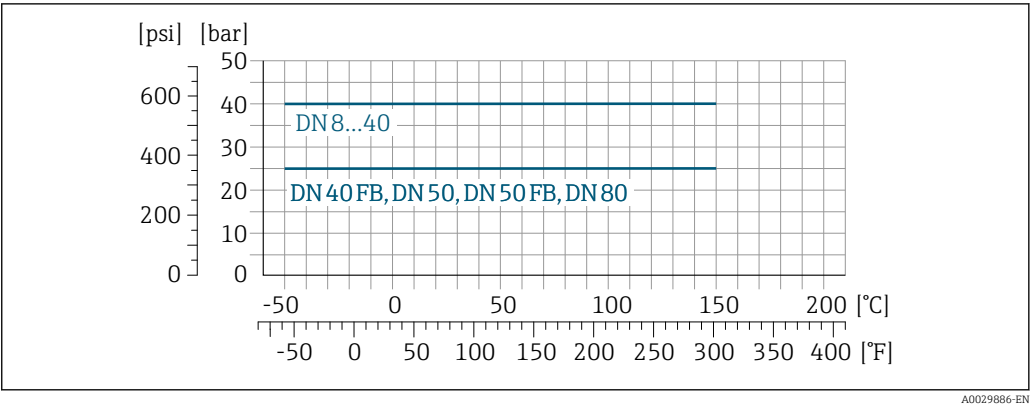
27 With connection material Grade 2 titanium
