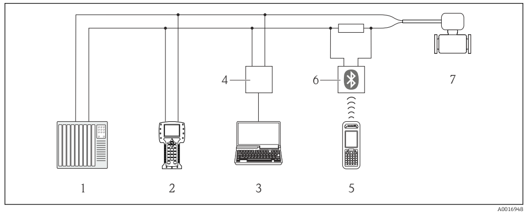
34 Options for remote operation via HART protocol
