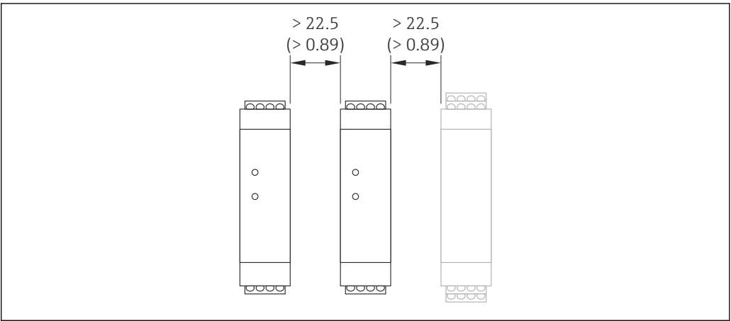
20 Minimum distance between additional Safety Barrier Promass 100 or other modules.Engineering unit mm (in)
