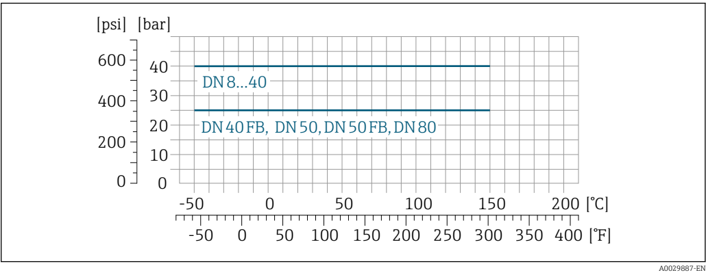
28 With connection material Grade 2 titanium
