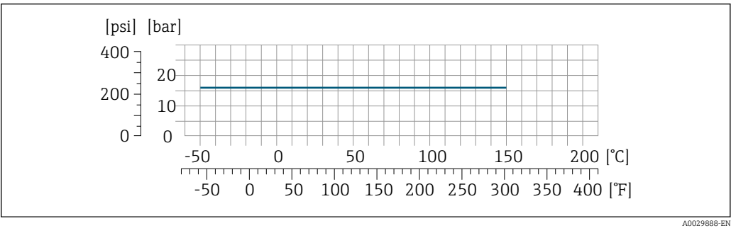
29 With connection material Grade 2 titanium
