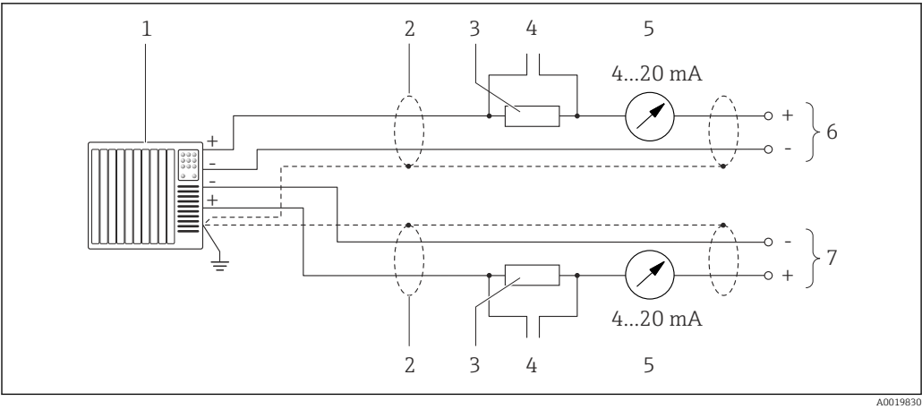
18 Connection example for HART input (master mode) via current output (active) 1 Automation system with current input (e.g. PLC). Prerequisite: automation system with HART version 6, HART commands 113 and 114 can be processed. 2 Cable shield, observe cable specifications 3 Resistor for HART communication ( \geq 250 \Omega ): observe maximum load 4 Connection for HART operating devices 5 Analog display unit 6 Transmitter 7 Sensor for external measured variable
