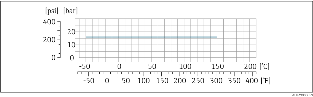
30 With connection material Grade 2 titanium
