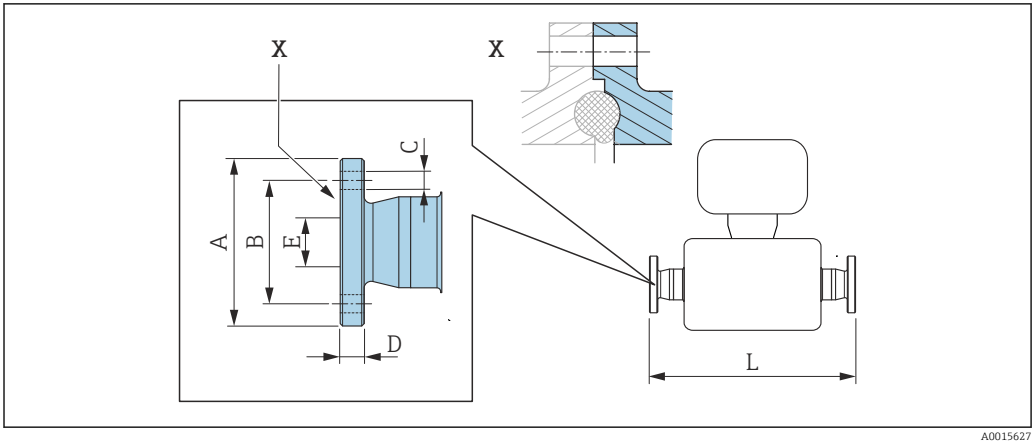
33 Detail X: Asymmetrical process connection; the part shown in gray is provided by the supplier.
