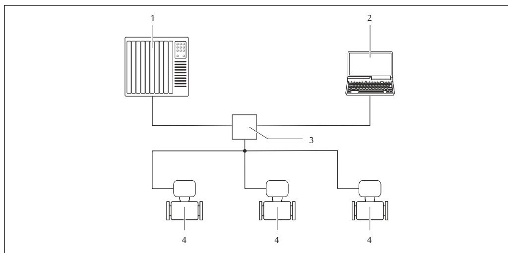
39 Options for remote operation via PROFINET network
