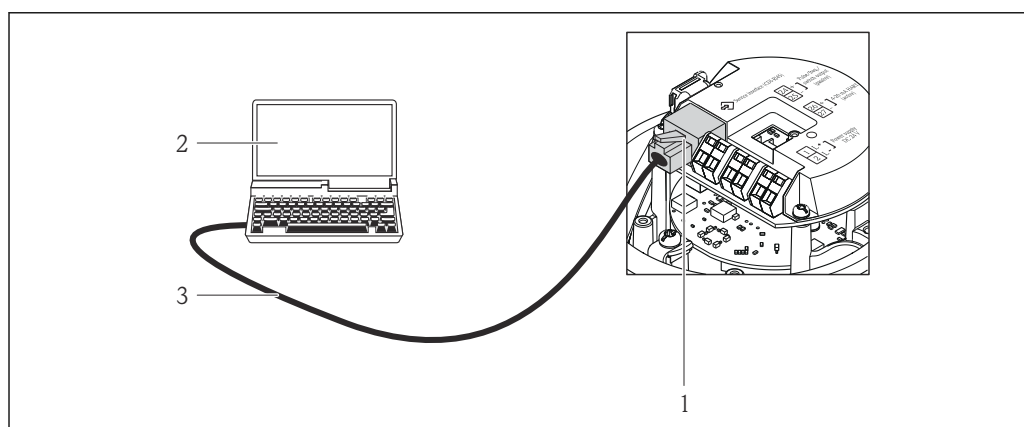
40 Connection for the order code for "Output", option B: 4-20 mA HART, pulse/frequency/switch output
