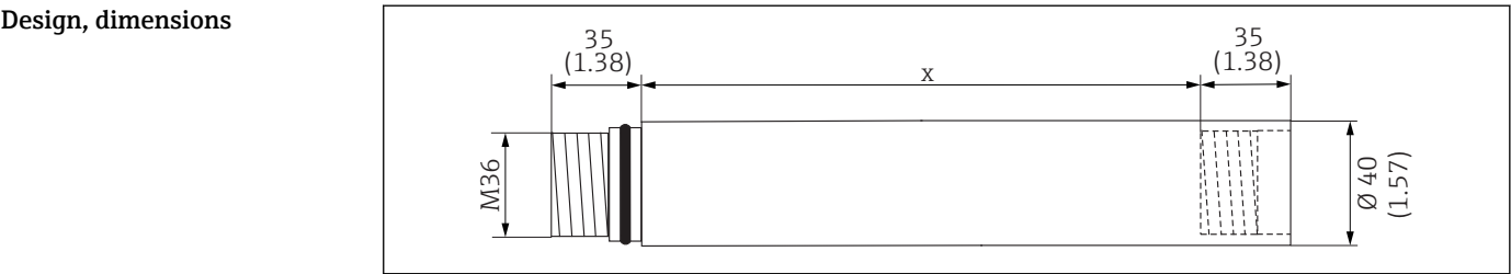
17 Immersion tube, stainless steel version
