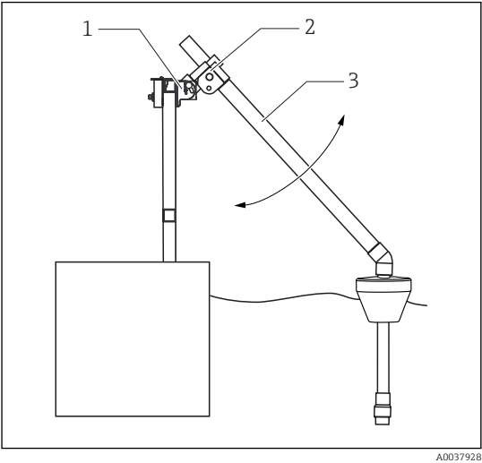
7 Float with pendulum holder
