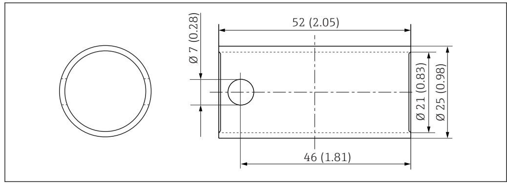
■ 23 Mounting tool. Dimensions: mm (in)
