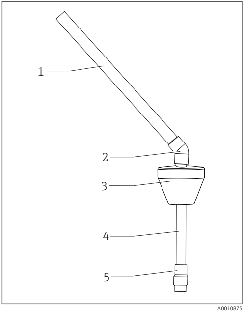
12 CYA112 with float
