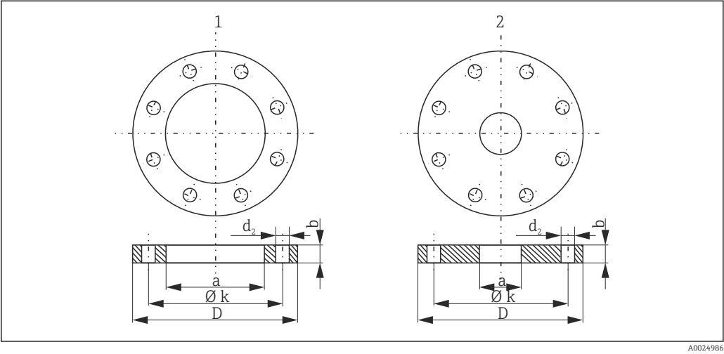
16 Flange dimensions
