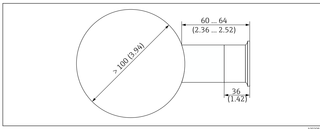
22 Pipe connection with weld-in adapter. Dimensions: mm (in)
