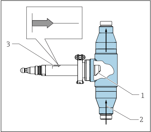
7 Sensor orientation
