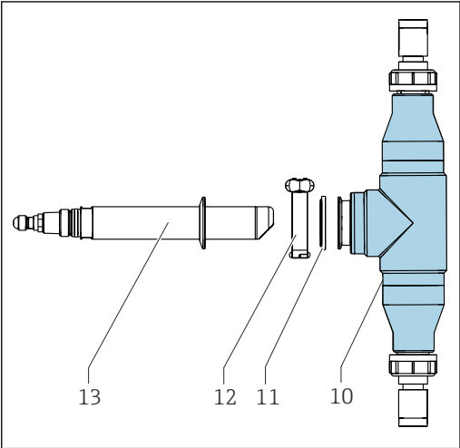
7 Sensor orientation
