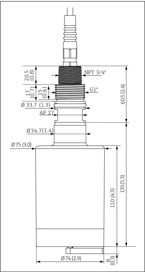
10 Dimensions for sensor with wiper. Dimensions: mm (in)
