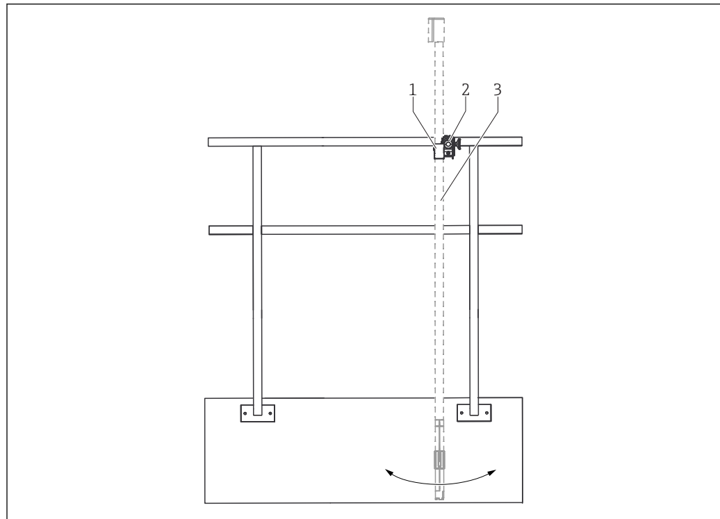
14 Pendulum holder on rail with immersion pipe
