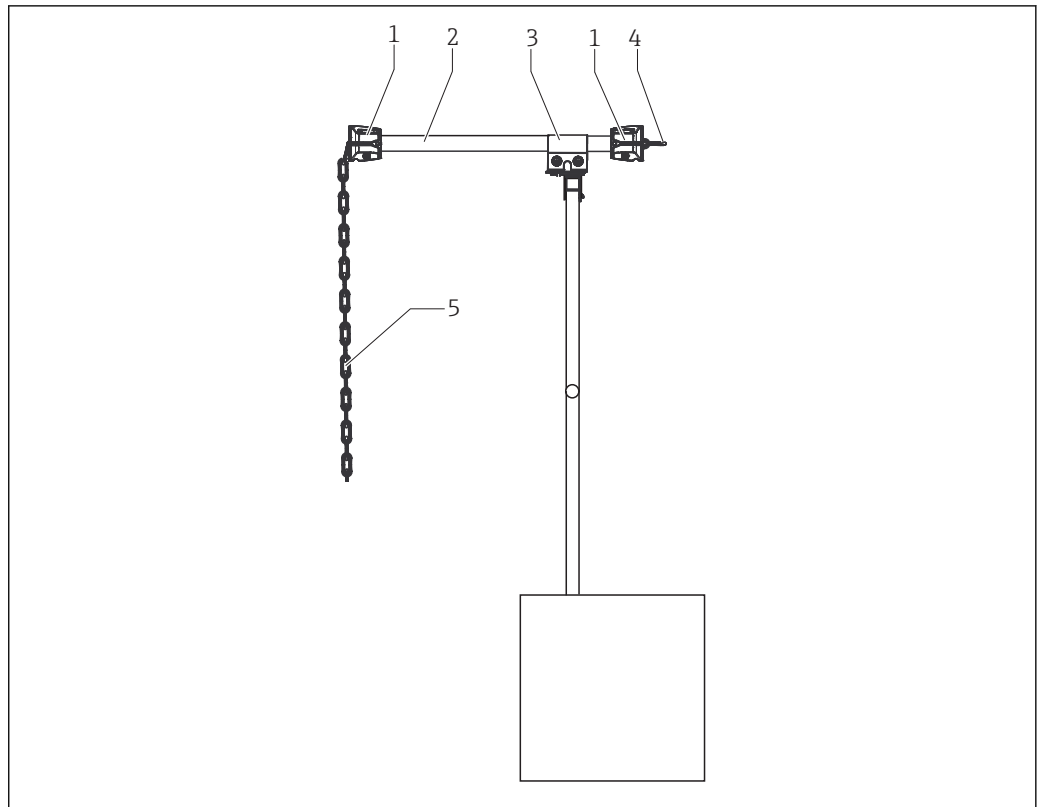
11 Transverse pipe on rail with chain retainer
