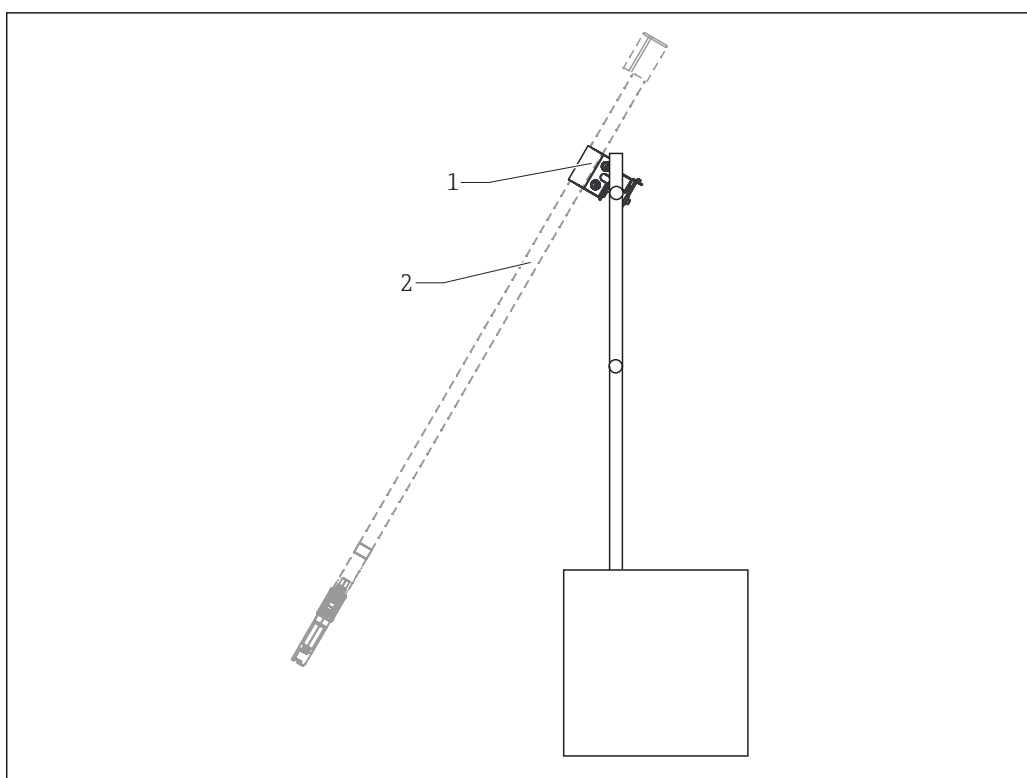
Rail mounting with angled position of immersion pipe
