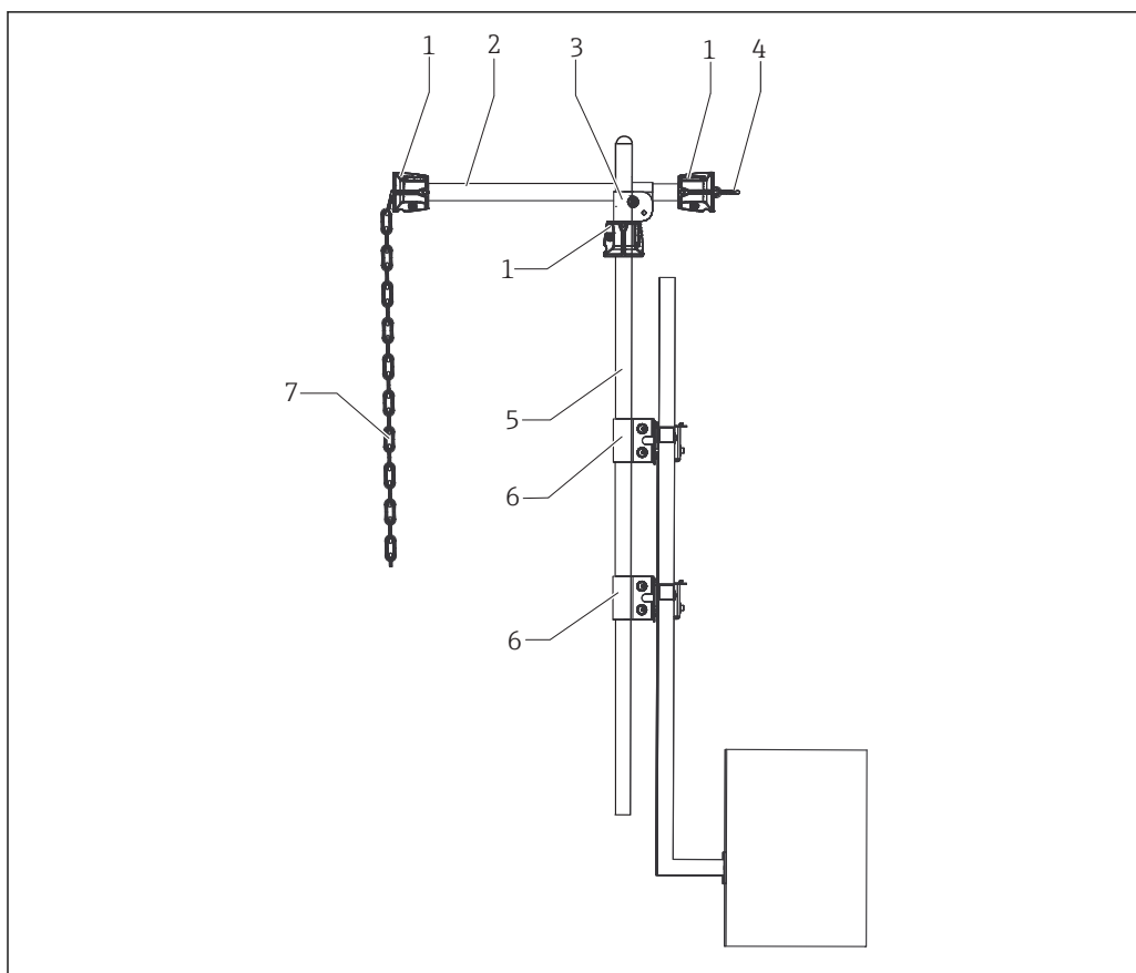
Main pipe on rail with chain retainer
