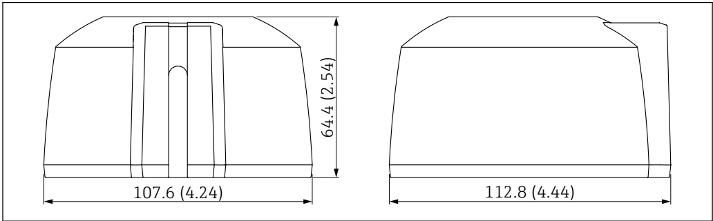
30 Dimensions for protective cover with cable entry at the side. Unit of measurement mm (in)
