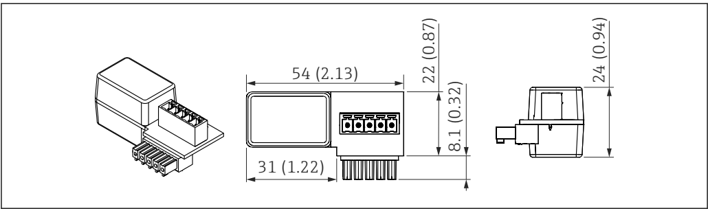
61 Dimensions of HART communication resistor. Unit of measurement mm (in)
