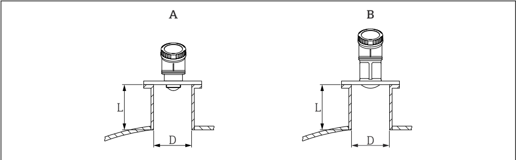
12 Nozzle installation
